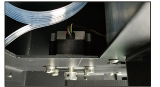
Step motor
